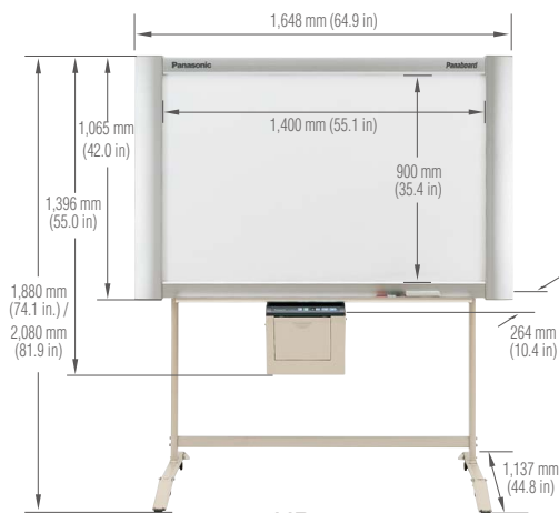
UB-7325 4-Screen Standard size (Stand option)
