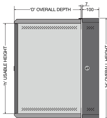
SIDE VIEW - RHS
